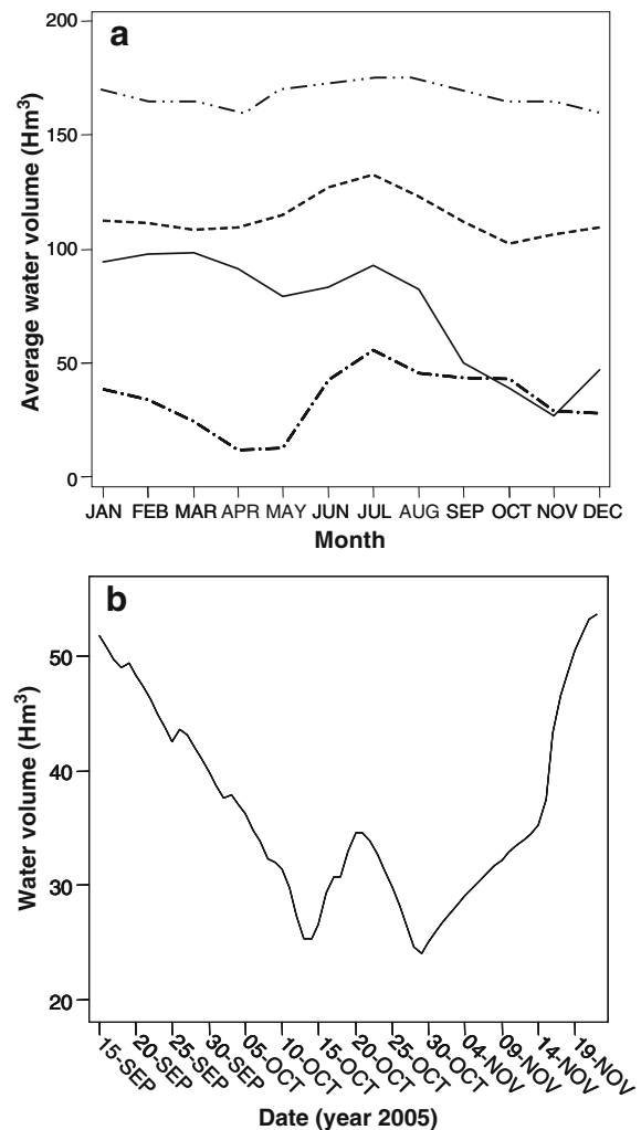
Fig. 1 a Maximum (— · — ·), mean (— — —), and minimum (— — —) monthly averages of water volume in Sau reservoir during 39 years (between January 1966 and December 2004) and the mean for 2005 (year of the partial drawdown, which started in September). b Variation of the water volume in Sau reservoir during the drawdown
